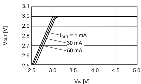
S-1112B30 ( T_a=25^\circ\text{C} )
