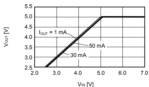
S-1112B50 ( T_a=25^\circ\text{C} )
