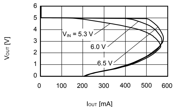
S-1112B50 ( T_a=25^\circ\text{C} )
