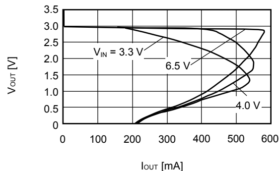
S-1112B30 ( T_a=25^\circ\text{C} )
