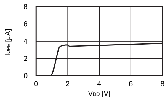
1.2 I_{OPE} - V_{DD}
