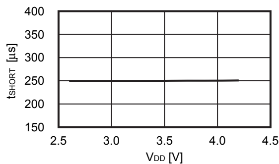
2. 14 t_{SHORT} - V_{DD}
