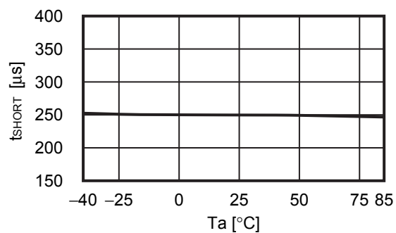
2. 15 t_{SHORT} - T_a
