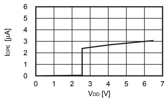
1.3 I_{OPE} - V_{DD}
