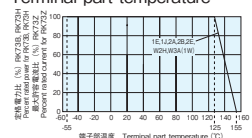
RK73B・RK73H・RK73Z-RT端子部温度 Terminal part temperature
