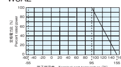
RK73B・RK73H-RT端子部温度 Terminal part temperature W3A2
