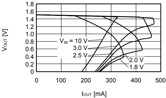
S-1200B50 (Ta=+25°C)
