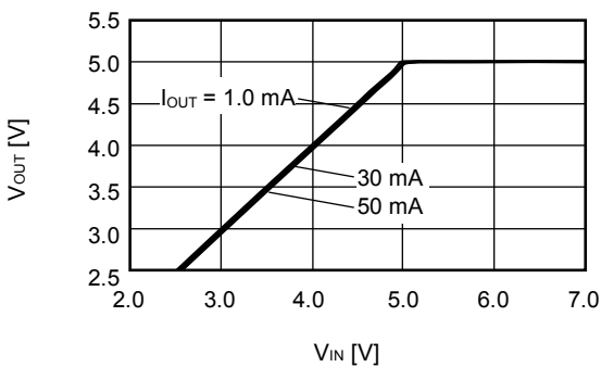
S-1200B50 (Ta=+25°C)
