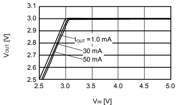
S-1200B30 (Ta=+25°C)
