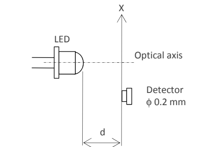
Measurement setup of light intensity distribution
