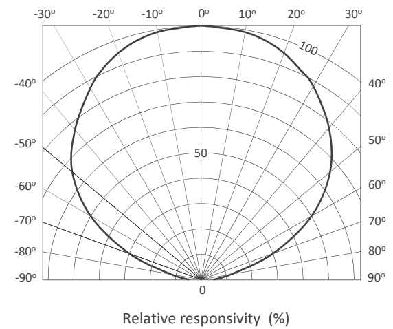
Directivity
