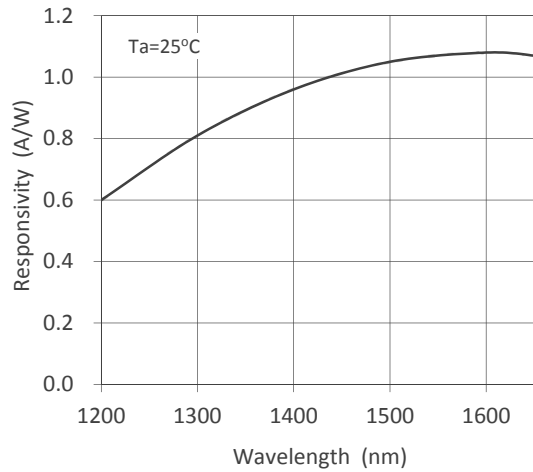
Spectral Responsivity
