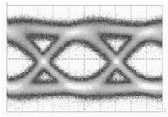
Hor. 50ps/div, Ver. 2.5mV/div, Pi=-20dBm
