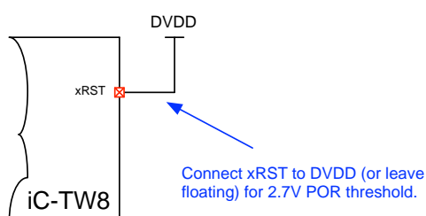
Figure 17: Setting the Power-On-Reset Threshold
