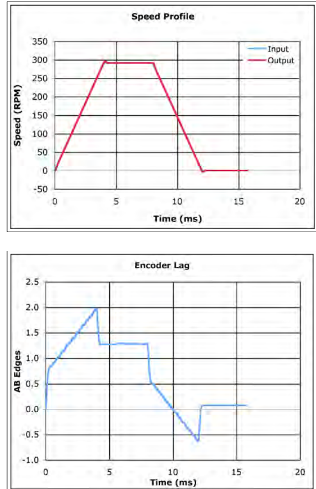
Figure 12: Typical Encoder Performance Graphs
