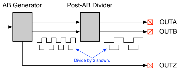
Figure 35: Post-AB Divider
