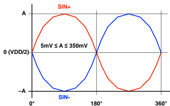
Figure 4: Differential Sensor Signal Inputs
