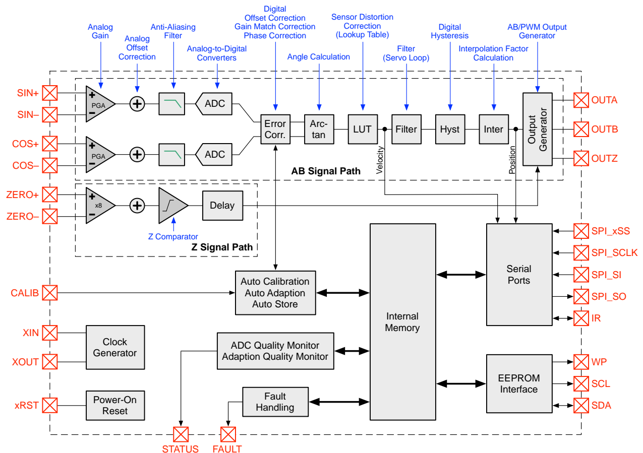
Figure 2: Block Diagram
