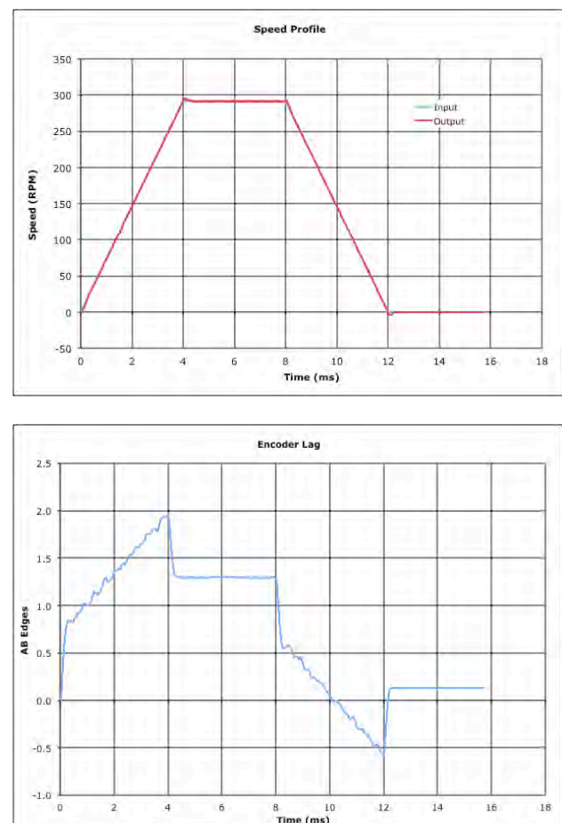
Figure 21: Typical Encoder Performance Graphs
