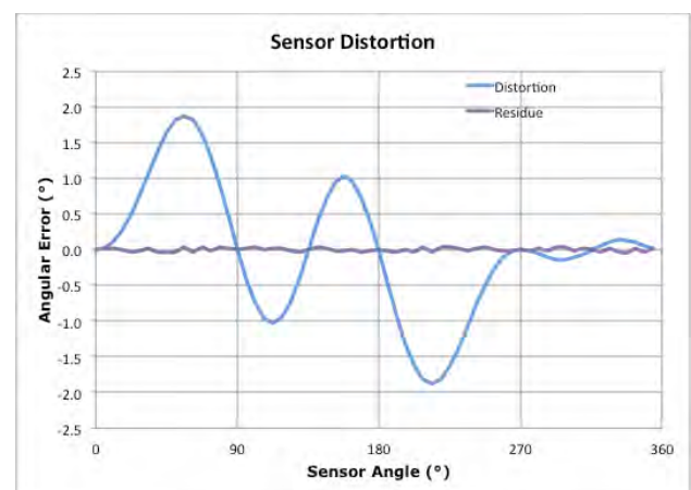
Figure 40: Sensor Distortion
