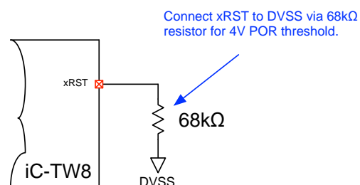
Figure 17: Setting the Power-On-Reset Threshold
