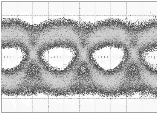
Hor. 500ps/div, Ver. 2mV/div, Pi=-31dBm, BR=622Mbps
