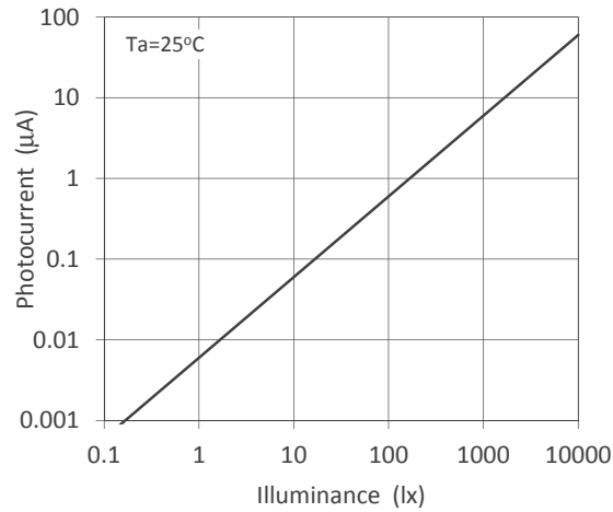
Photocurrent - Illuminance
