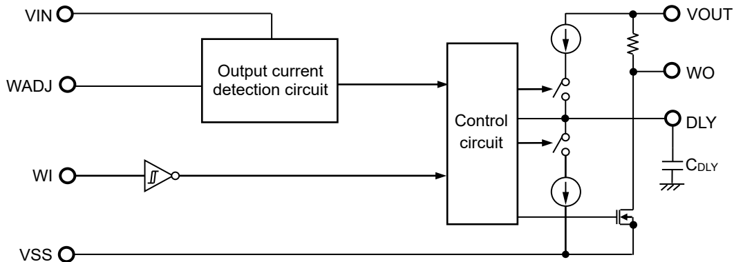
Figure 48 Operation of Watchdog Timer Block
