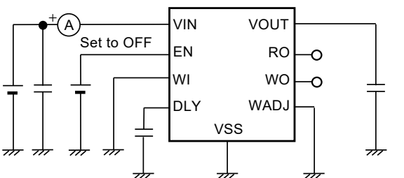
Figure 32 Test Circuit 10
