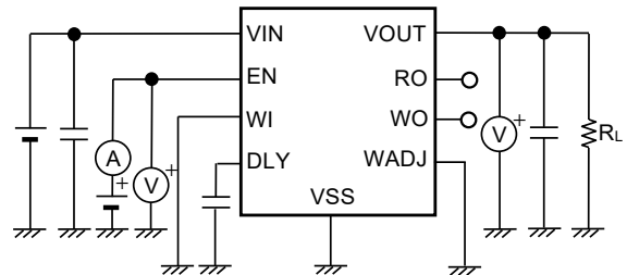
Figure 26 Test Circuit 4
