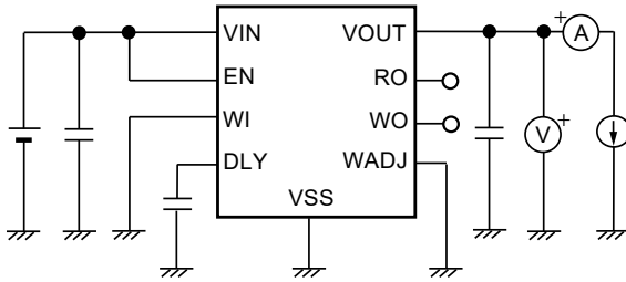
Figure 23 Test Circuit 1
