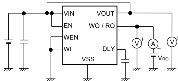
Figure 18 Test Circuit 6
