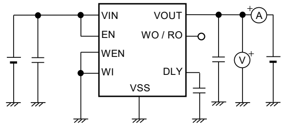
Figure 14 Test Circuit 2
