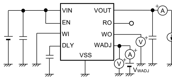
Figure 30 Test Circuit 8
