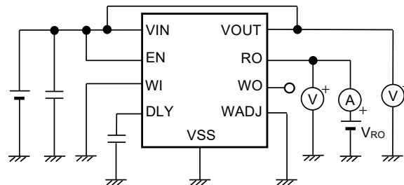
Figure 28 Test Circuit 6
