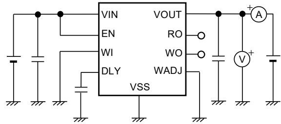
Figure 24 Test Circuit 2
