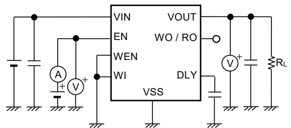
Figure 16 Test Circuit 4
