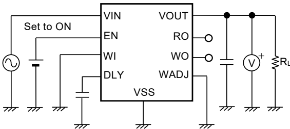
Figure 25 Test Circuit 3
