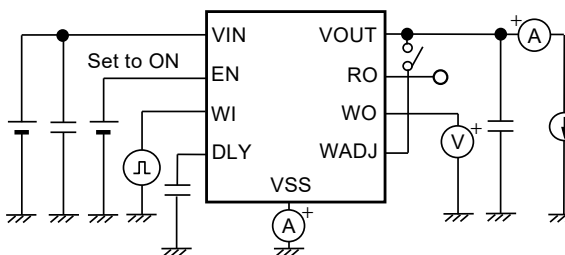
Figure 31 Test Circuit 9
