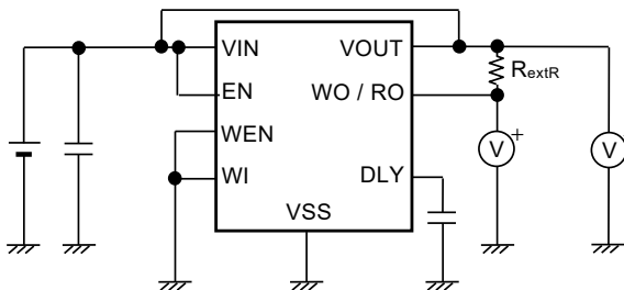
Figure 17 Test Circuit 5
