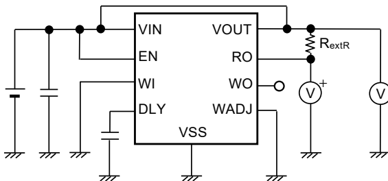
Figure 27 Test Circuit 5
