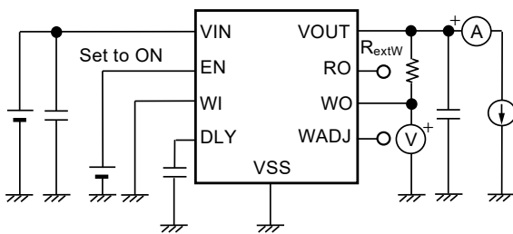
Figure 29 Test Circuit 7
