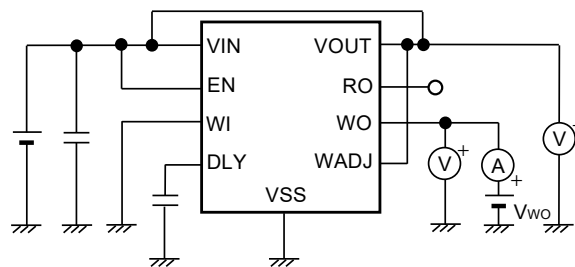
Figure 34 Test Circuit 12
