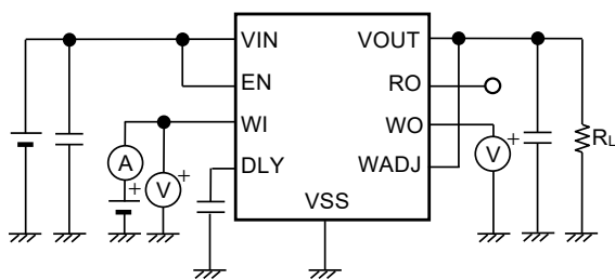
Figure 33 Test Circuit 11
