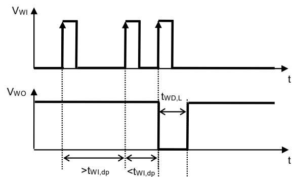
Figure 12 Watchdog Double-pulse Detection Time
