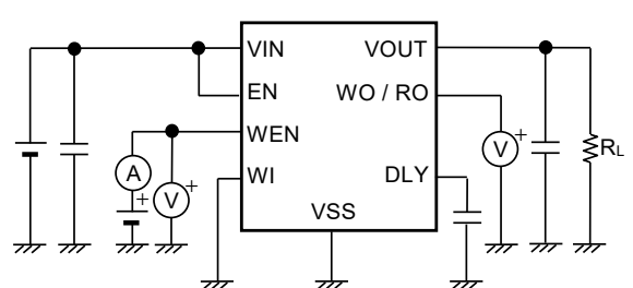
Figure 20 Test Circuit 8
