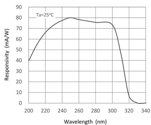
Spectral Responsivity
